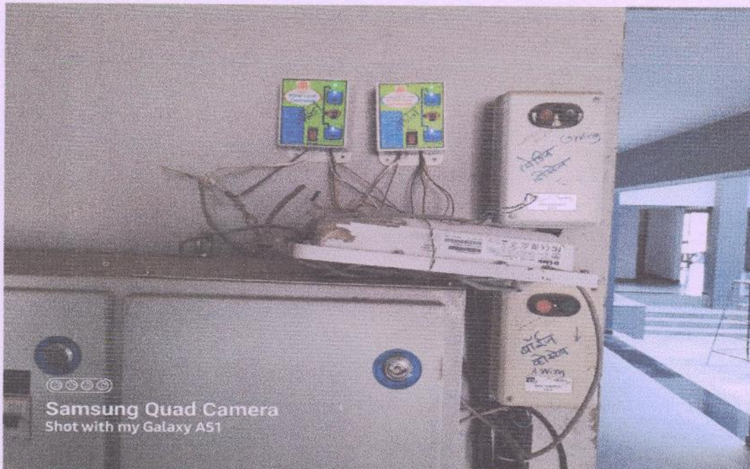
Sensor base automatic on / off for water tanks
